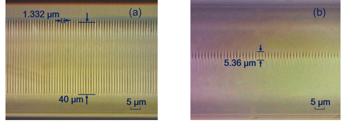
Fig. 2. (a) The top view and (b) side view photomicrographs of fabricated SFBG.
