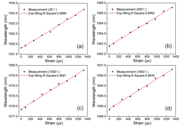
Fig. 7. (a)-(d) The relationship between resonance wavelength and strain of SFBG at different temperature.
